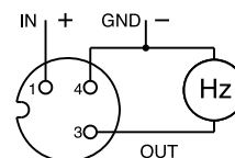
Frequency output
