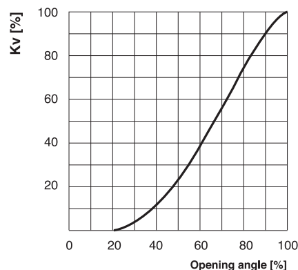
Flow characteristic
