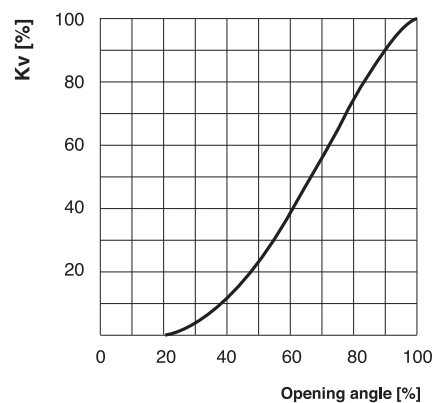
Flow characteristic
